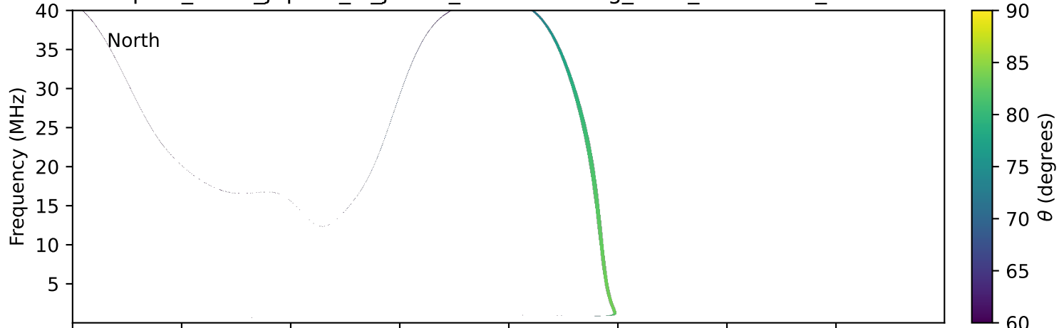
expres_earth_jupiter_io_jrm33_lossc-wid1deg_3kev_19980507_v11.cdf
