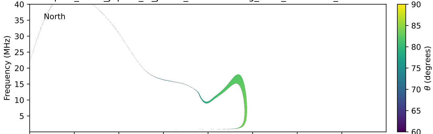
expres_earth_jupiter_io_jrm09_lossc-wid1deg_3kev_19980523_v11.cdf
