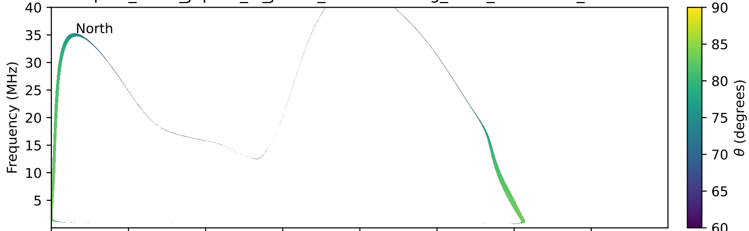
expres_earth_jupiter_io_jrm09_lossc-wid1deg_3kev_19980521_v11.cdf
