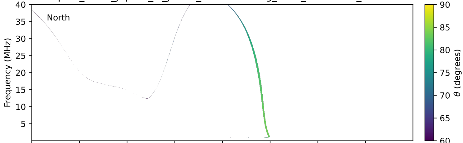
expres_earth_jupiter_io_jrm09_lossc-wid1deg_3kev_19980507_v11.cdf
