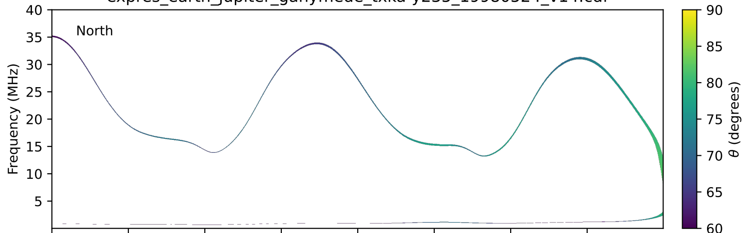
expres_earth_jupiter_ganymede_txka-y235_19980524_v14.cdf
