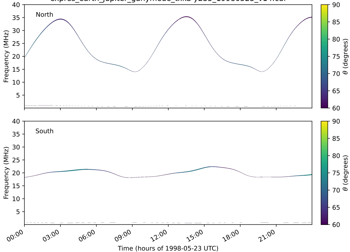
expres_earth_jupiter_ganymede_txka-y235_19980523_v14.cdf
