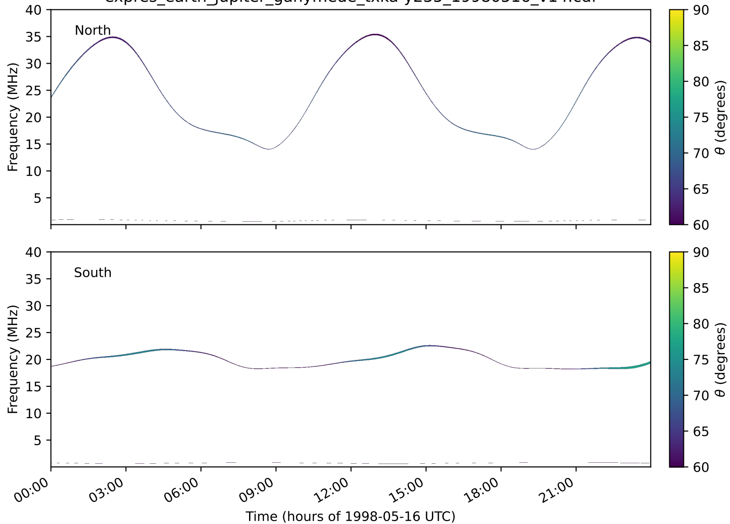
expres_earth_jupiter_ganymede_txka-y235_19980516_v14.cdf
