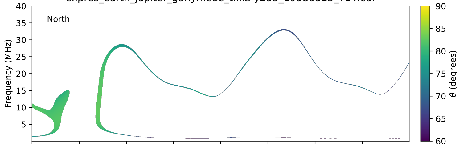
expres_earth_jupiter_ganymede_txka-y235_19980515_v14.cdf
