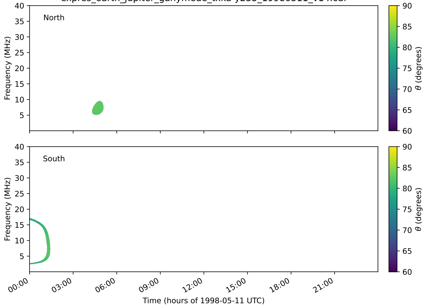
expres_earth_jupiter_ganymede_txka-y235_19980511_v14.cdf
