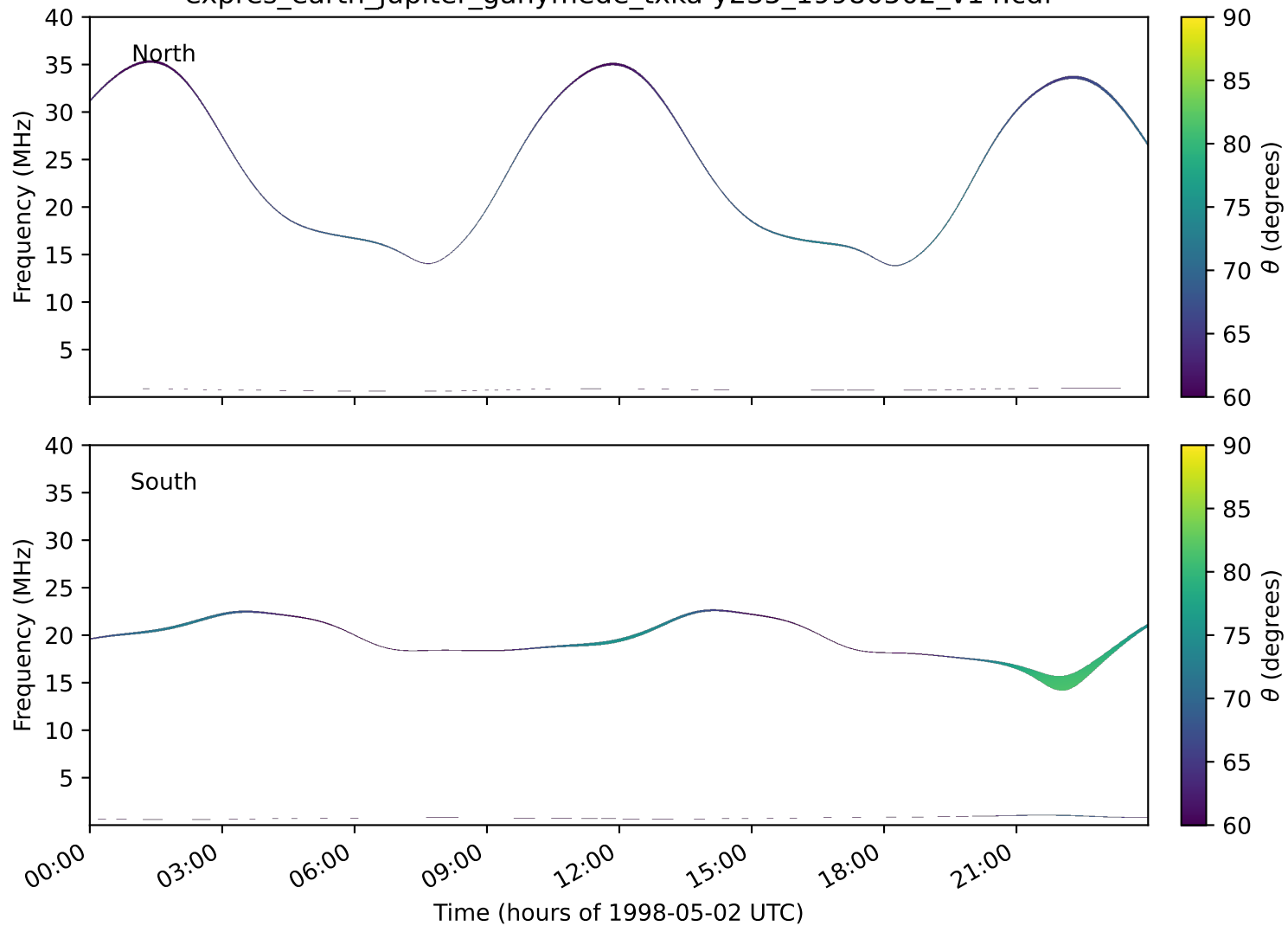
expres_earth_jupiter_ganymede_txka-y235_19980502_v14.cdf
