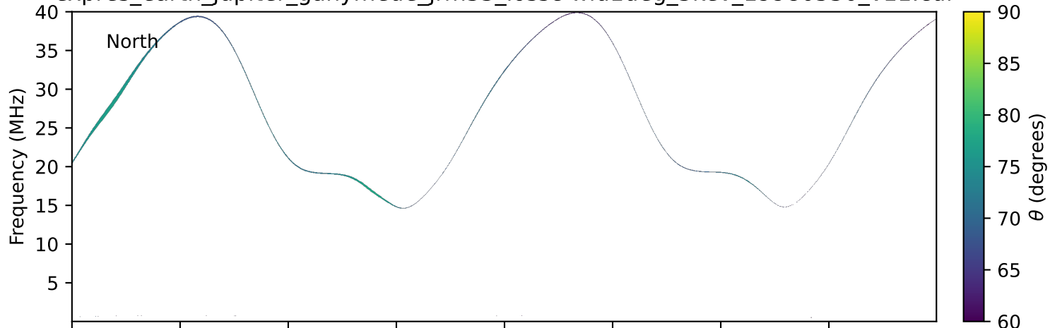
expres_earth_jupiter_ganymede_jrm33_lossc-wid1deg_3kev_19980530_v11.cdf
