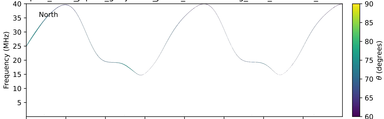
expres_earth_jupiter_ganymede_jrm33_lossc-wid1deg_3kev_19980523_v11.cdf
