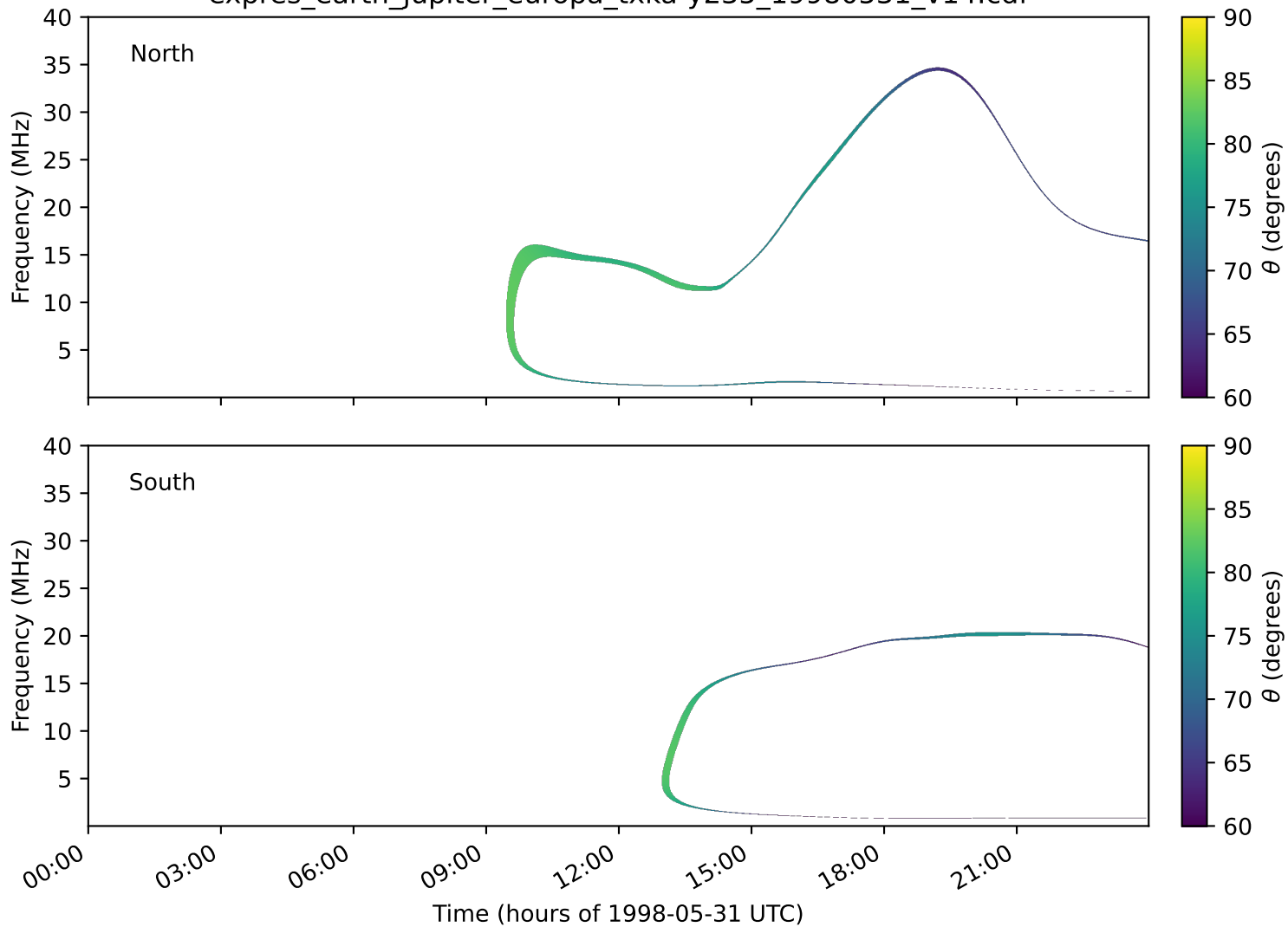
expres_earth_jupiter_europa_txka-y235_19980531_v14.cdf
