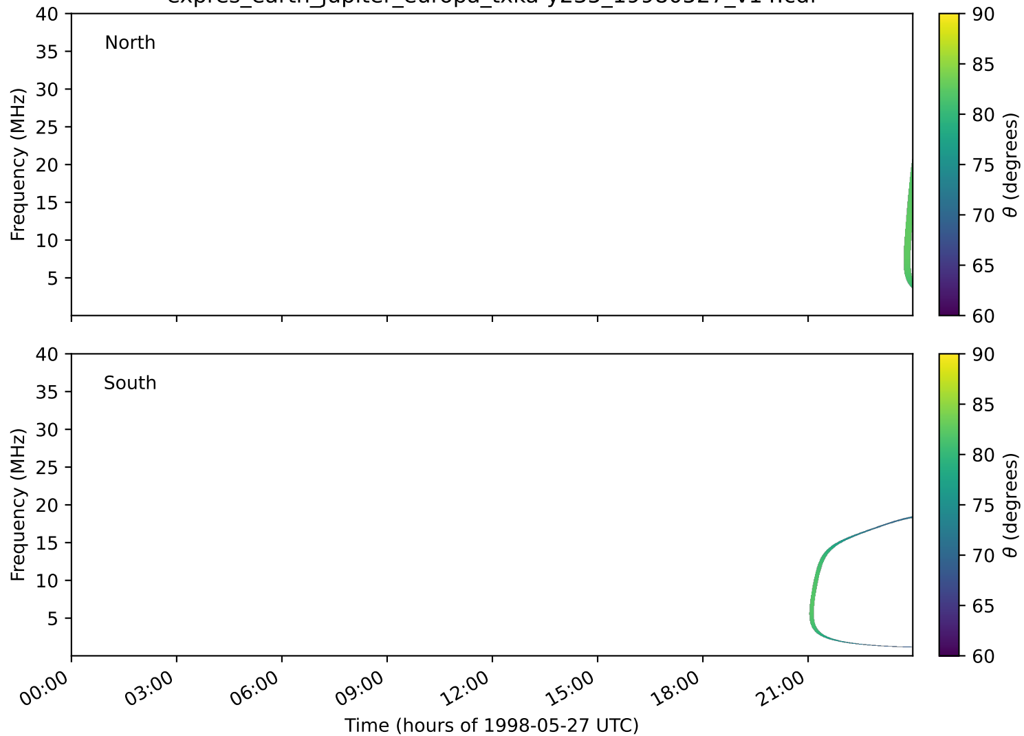
expres_earth_jupiter_europa_txka-y235_19980527_v14.cdf
