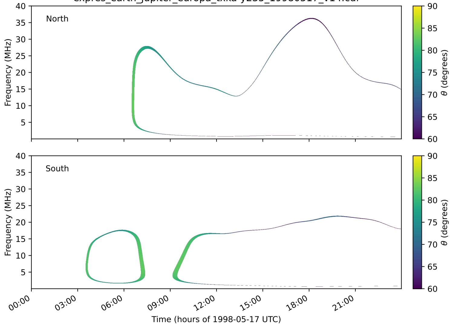
expres_earth_jupiter_europa_txka-y235_19980517_v14.cdf
