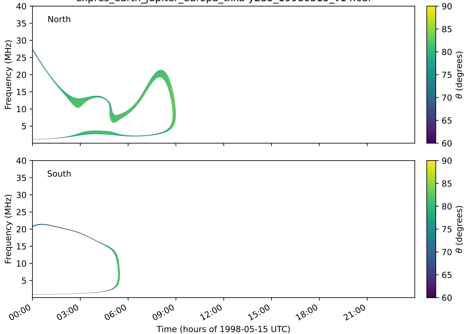
expres_earth_jupiter_europa_txka-y235_19980515_v14.cdf
