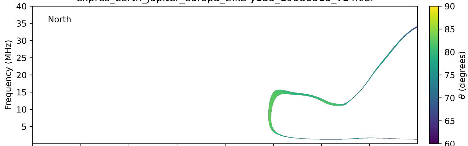
expres_earth_jupiter_europa_txka-y235_19980513_v14.cdf
