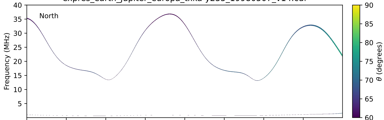
expres_earth_jupiter_europa_txka-y235_19980507_v14.cdf
