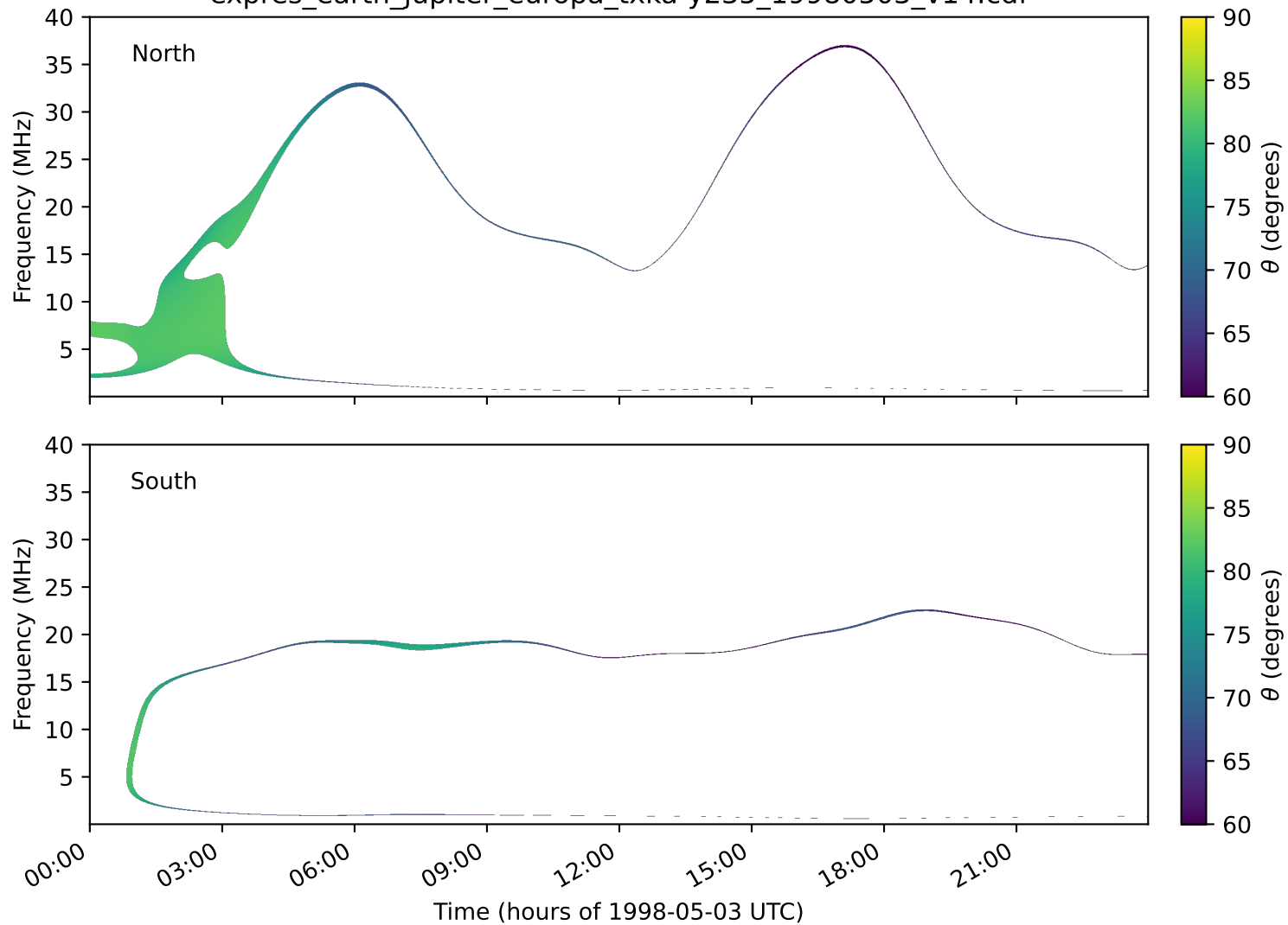
expres_earth_jupiter_europa_txka-y235_19980503_v14.cdf
