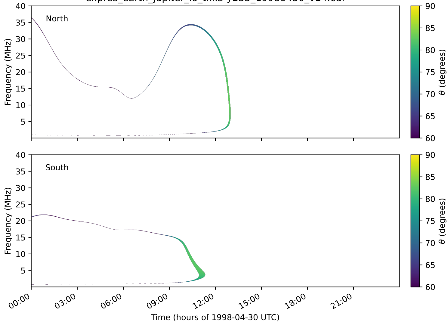
expres_earth_jupiter_io_txka-y235_19980430_v14.cdf
