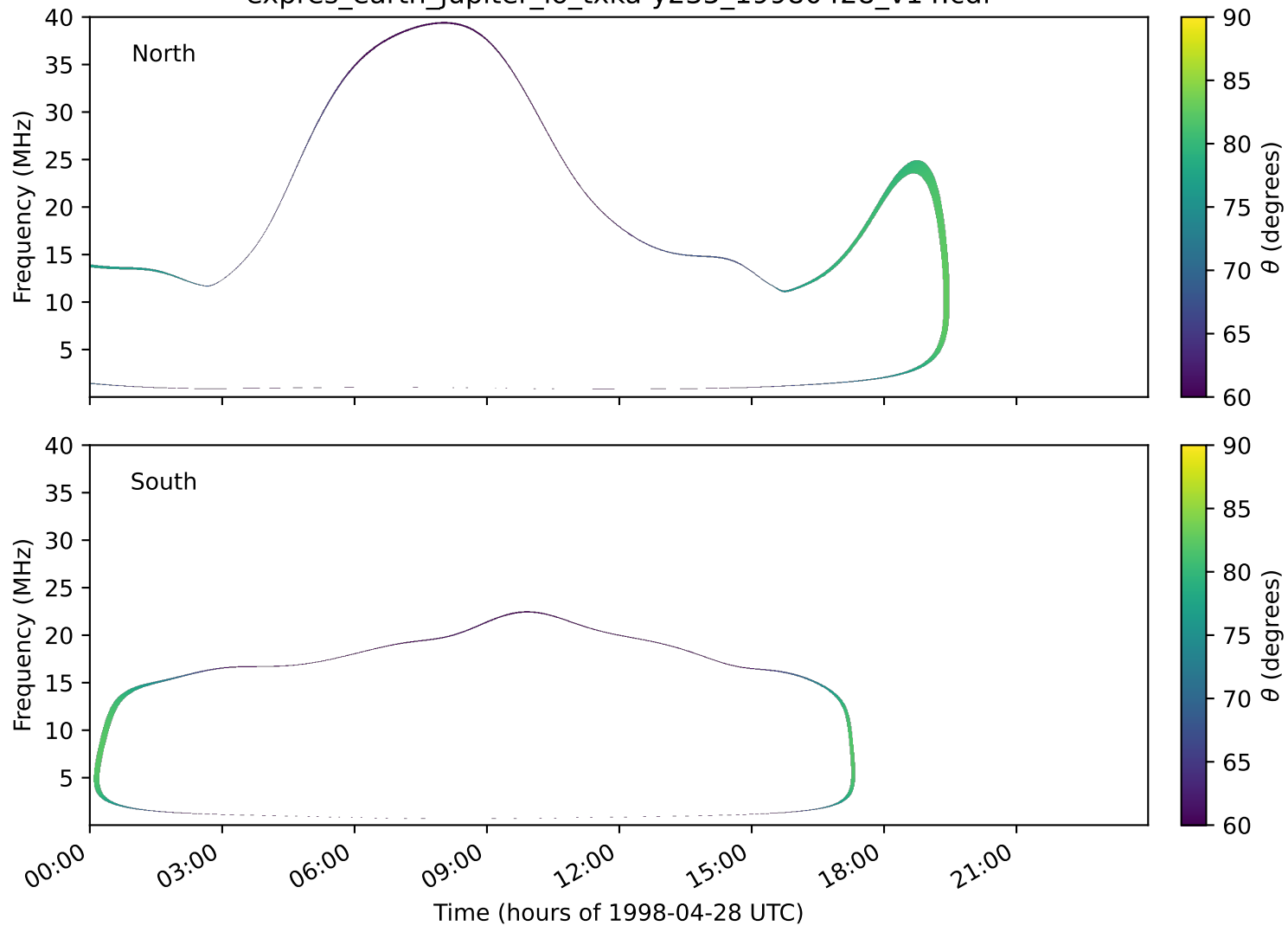
expres_earth_jupiter_io_txka-y235_19980428_v14.cdf
