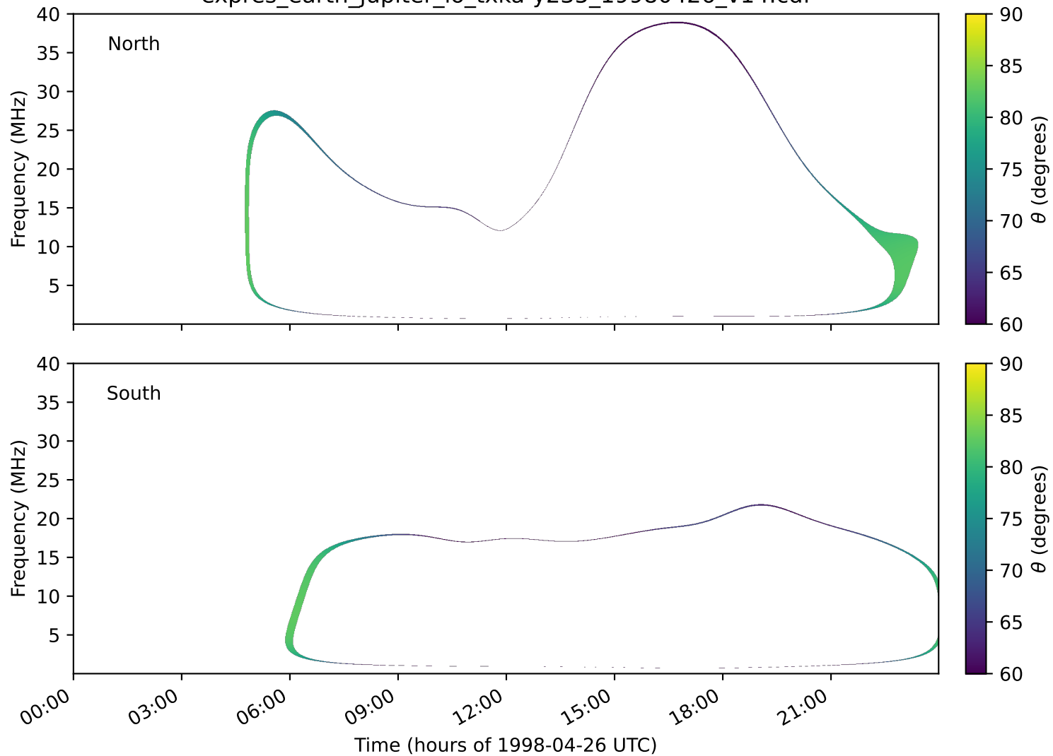
expres_earth_jupiter_io_txka-y235_19980426_v14.cdf
