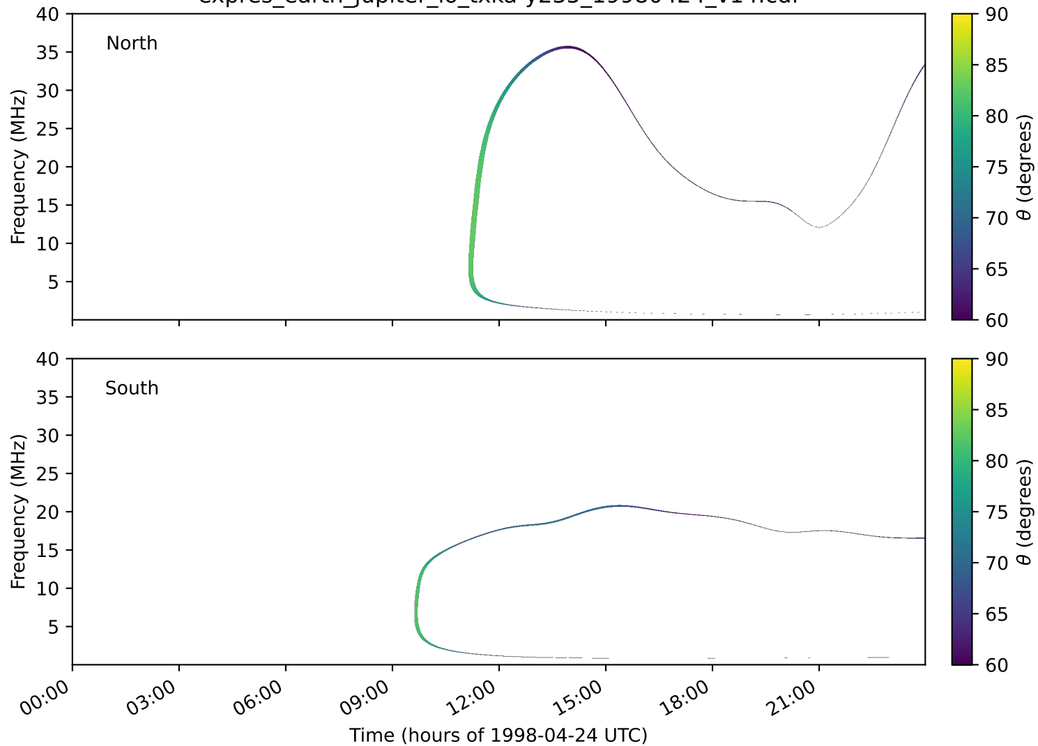
expres_earth_jupiter_io_txka-y235_19980424_v14.cdf
