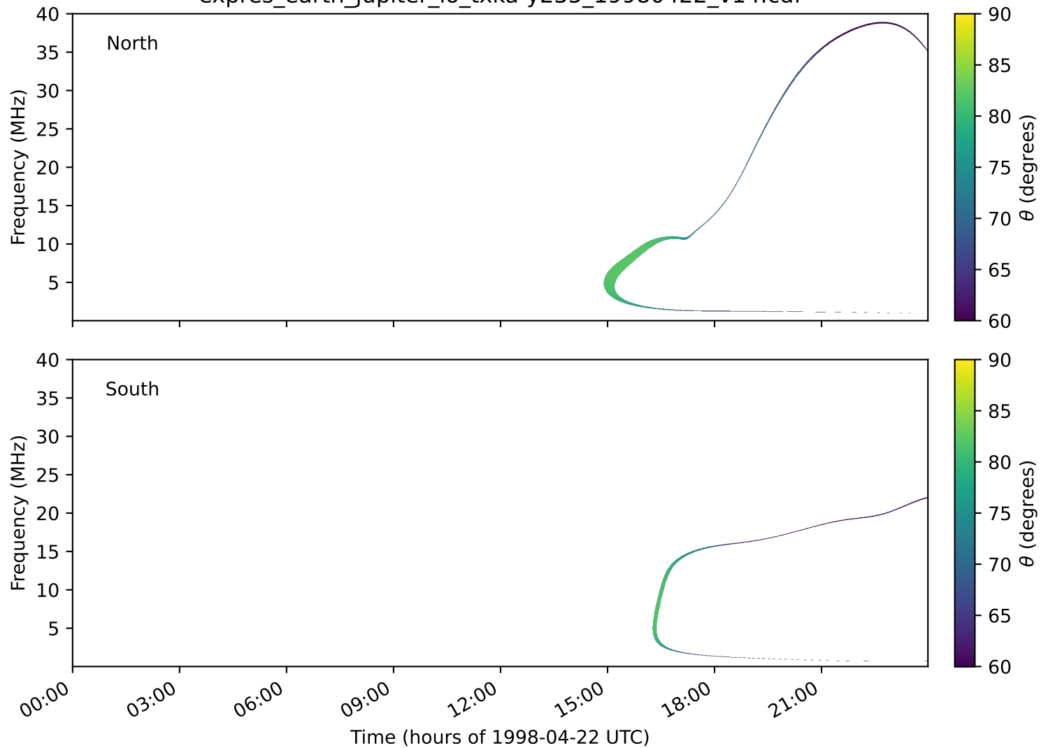
expres_earth_jupiter_io_txka-y235_19980422_v14.cdf
