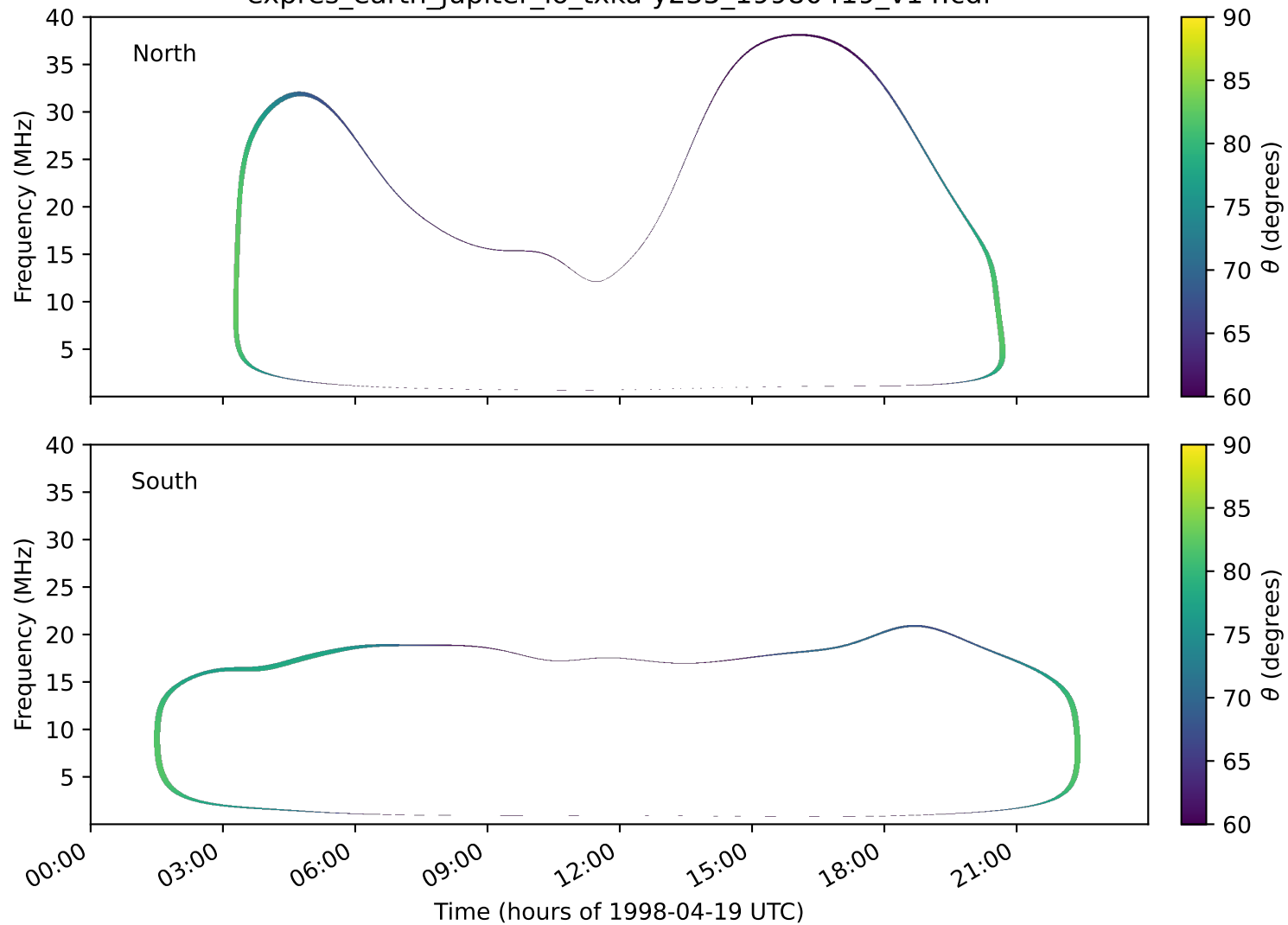
expres_earth_jupiter_io_txka-y235_19980419_v14.cdf
