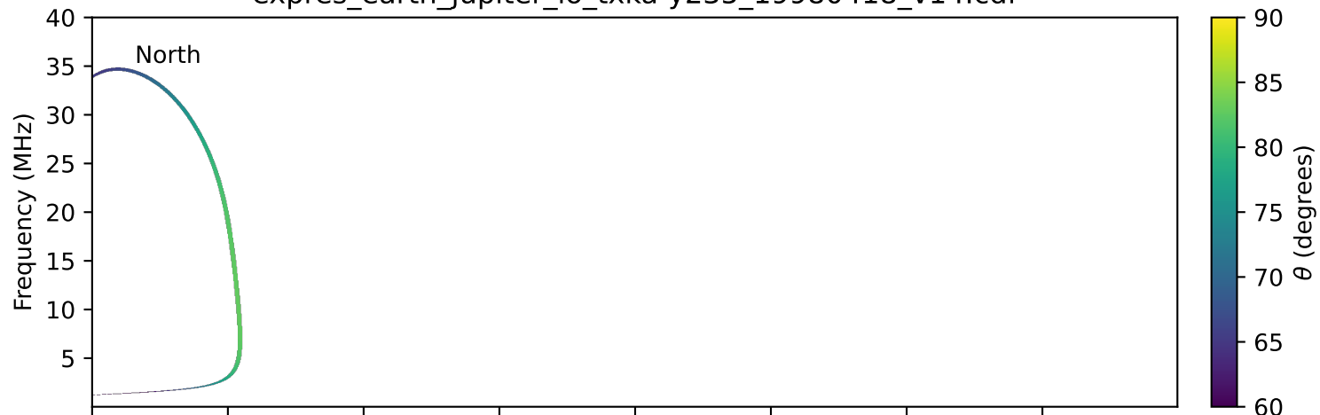
expres_earth_jupiter_io_txka-y235_19980418_v14.cdf
