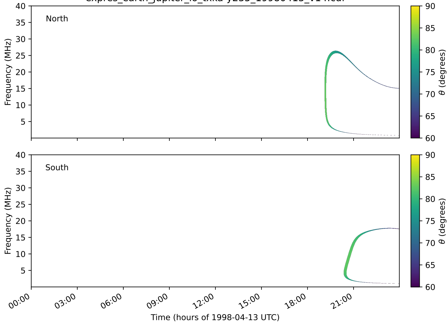
expres_earth_jupiter_io_txka-y235_19980413_v14.cdf
