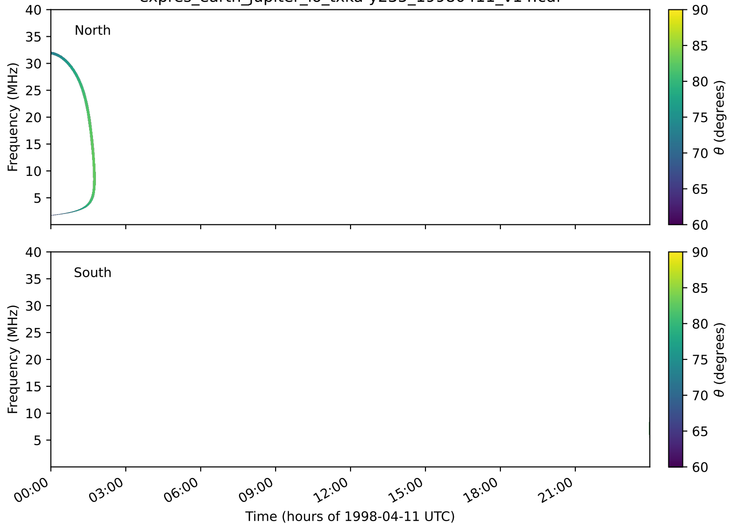
expres_earth_jupiter_io_txka-y235_19980411_v14.cdf
