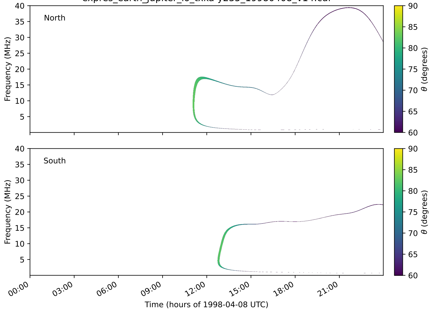
expres_earth_jupiter_io_txka-y235_19980408_v14.cdf
