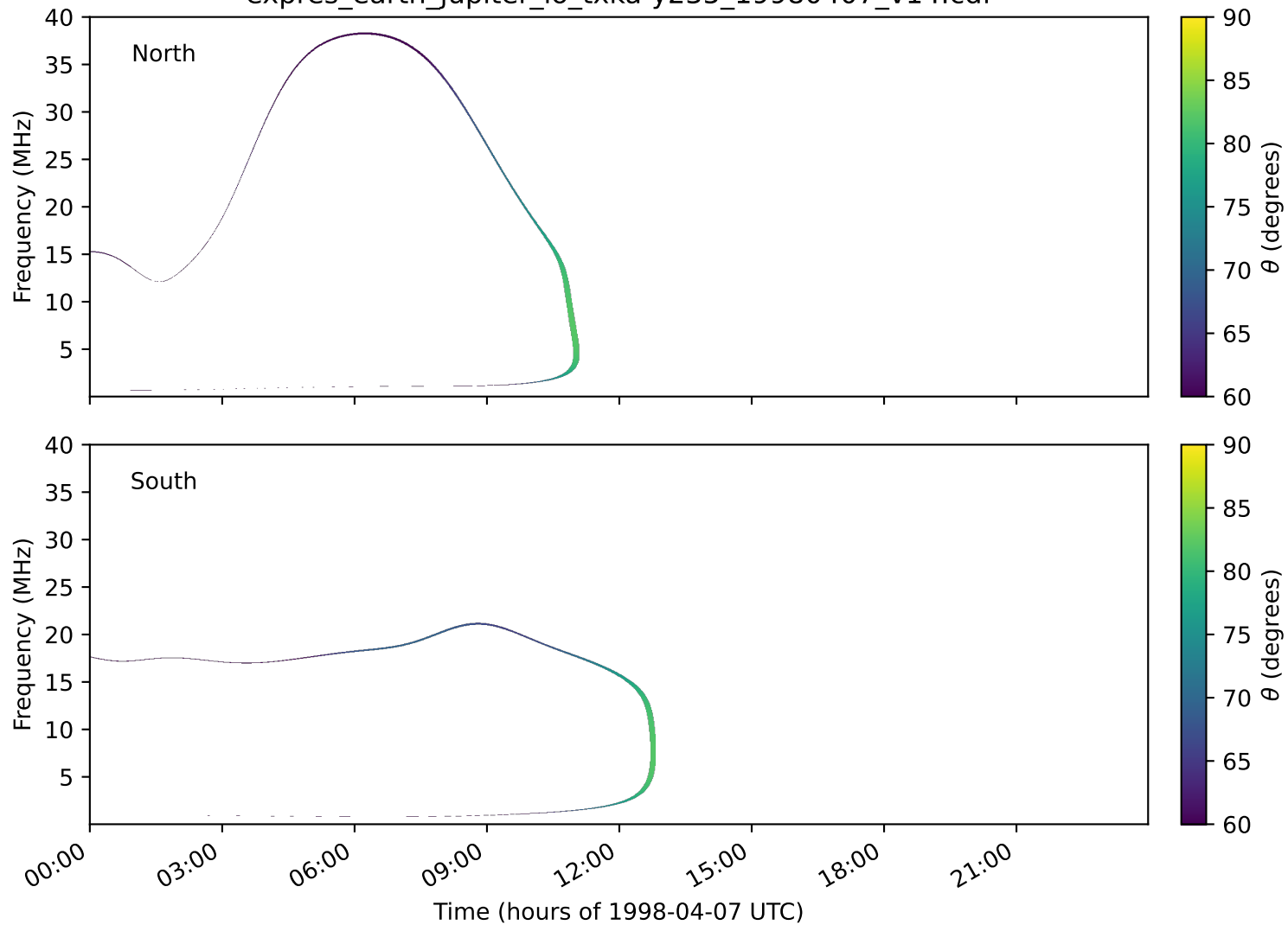
expres_earth_jupiter_io_txka-y235_19980407_v14.cdf
