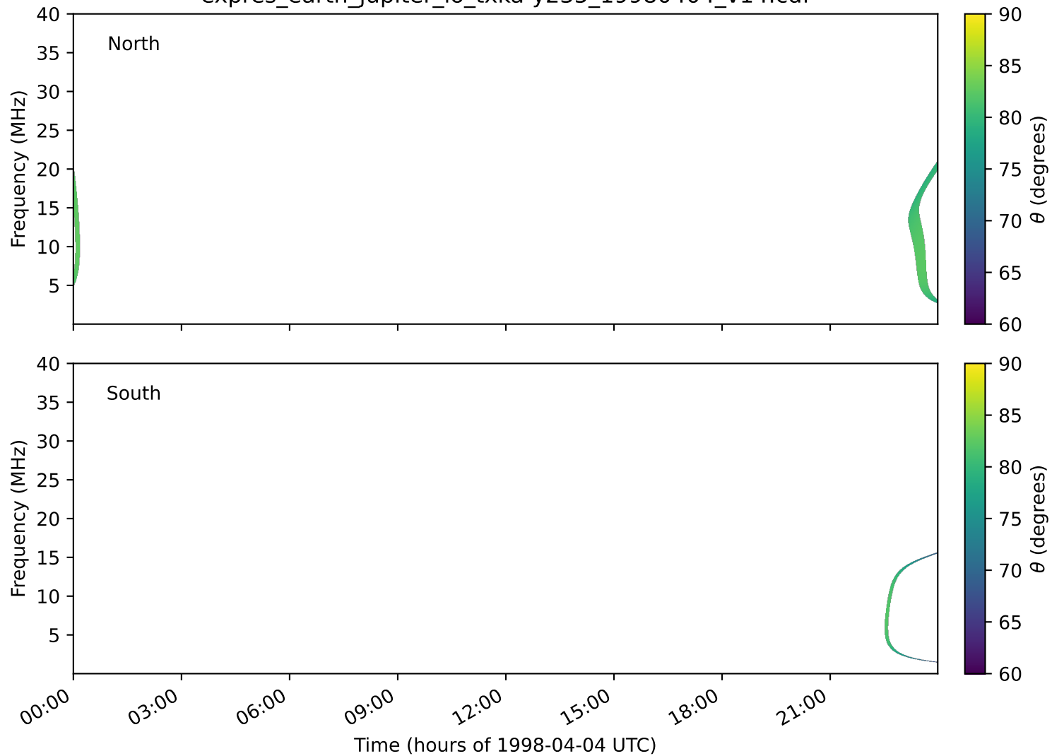
expres_earth_jupiter_io_txka-y235_19980404_v14.cdf
