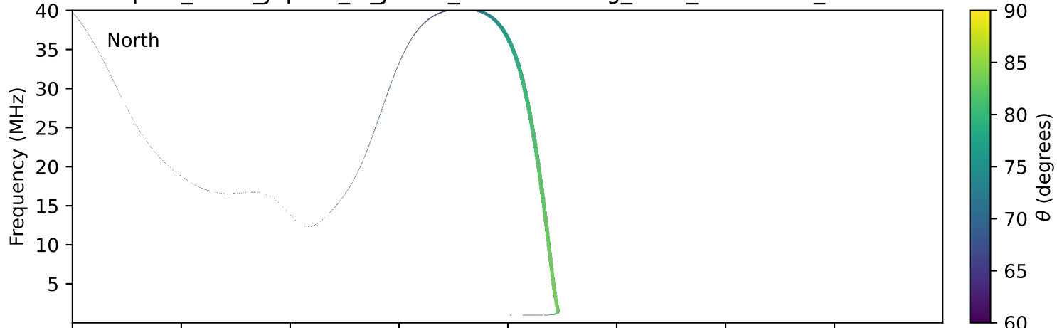
expres_earth_jupiter_io_jrm33_lossc-wid1deg_3kev_19980430_v11.cdf
