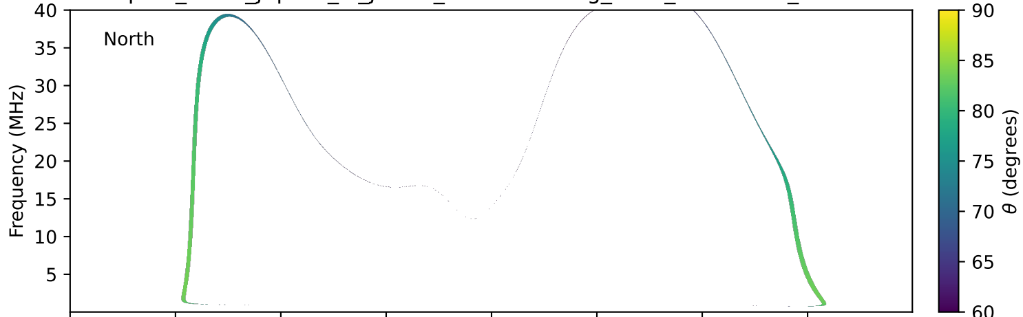
expres_earth_jupiter_io_jrm33_lossc-wid1deg_3kev_19980419_v11.cdf
