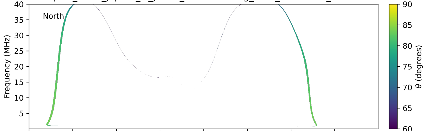
expres_earth_jupiter_io_jrm33_lossc-wid1deg_3kev_19980412_v11.cdf
