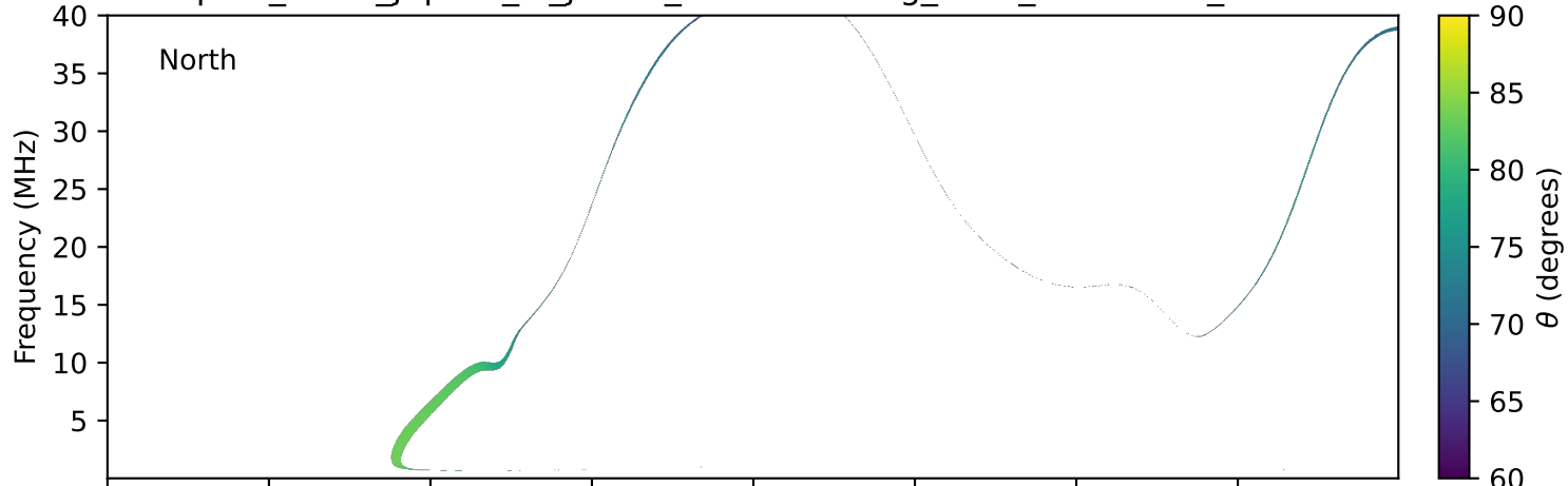
expres_earth_jupiter_io_jrm33_lossc-wid1deg_3kev_19980410_v11.cdf
