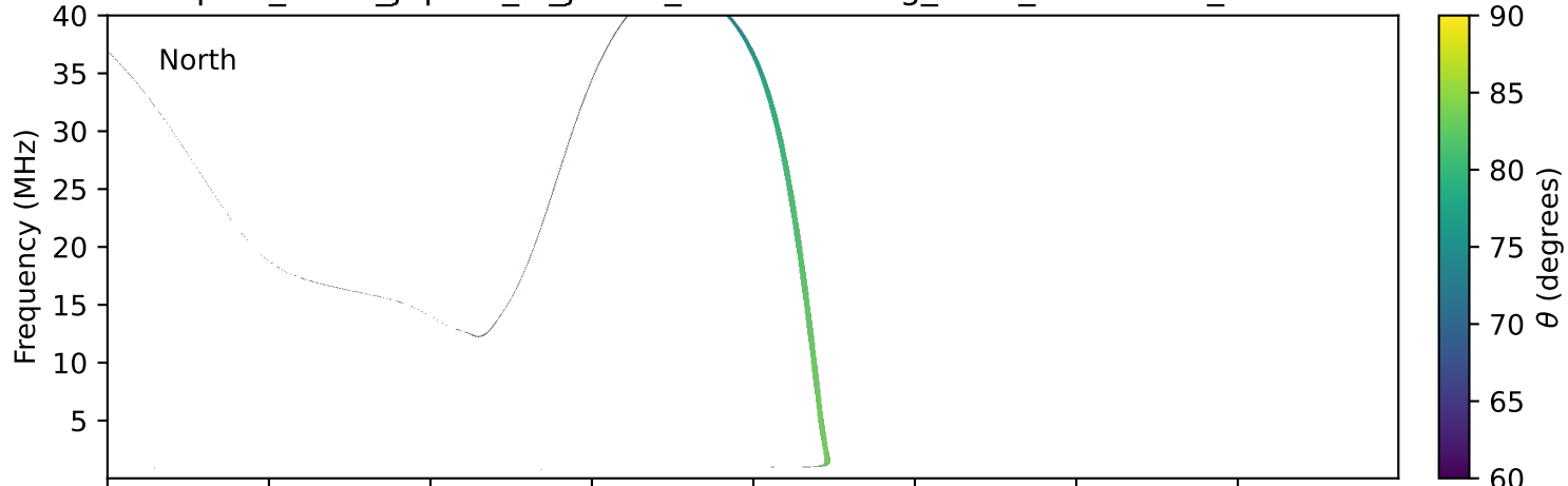
expres_earth_jupiter_io_jrm09_lossc-wid1deg_3kev_19980430_v11.cdf
