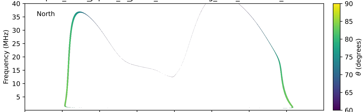
expres_earth_jupiter_io_jrm09_lossc-wid1deg_3kev_19980419_v11.cdf
