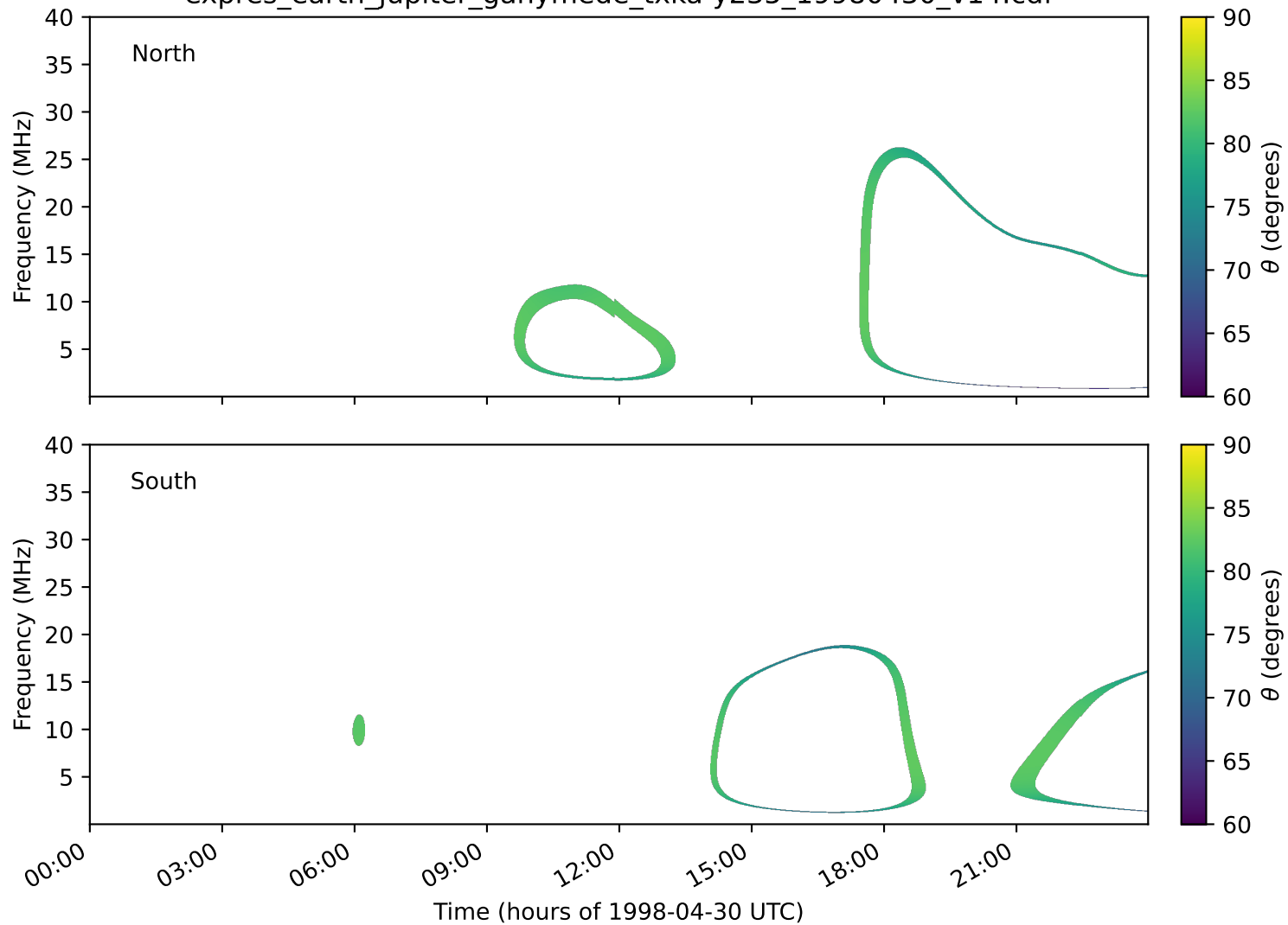
expres_earth_jupiter_ganymede_txka-y235_19980430_v14.cdf
