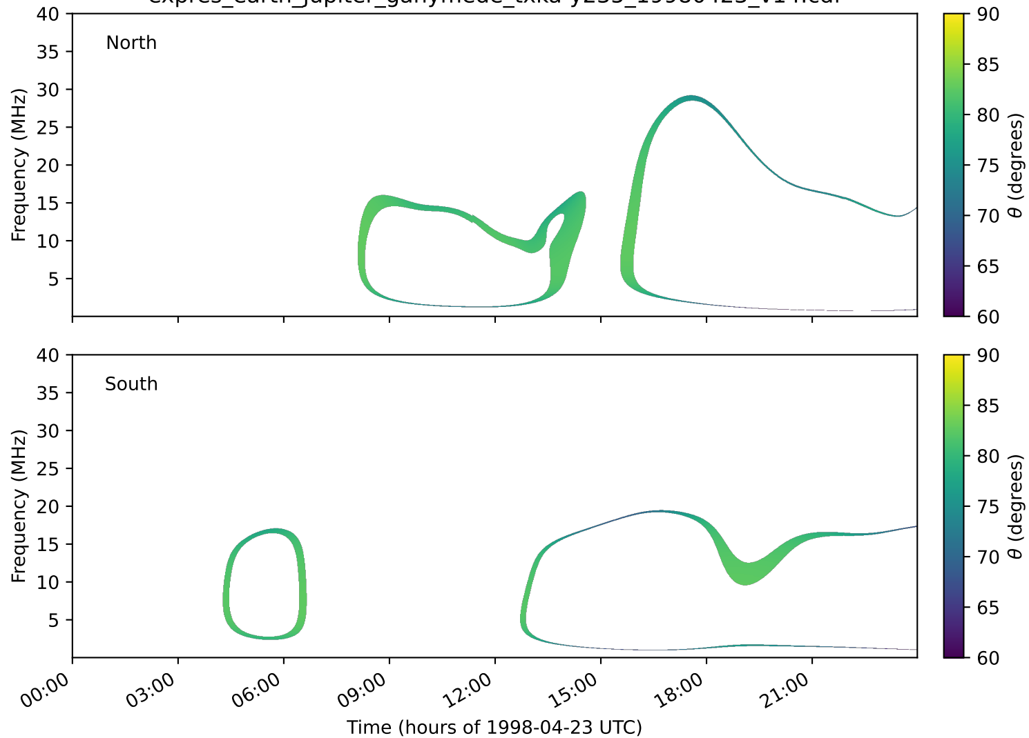
expres_earth_jupiter_ganymede_txka-y235_19980423_v14.cdf
