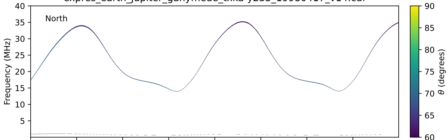
expres_earth_jupiter_ganymede_txka-y235_19980417_v14.cdf
