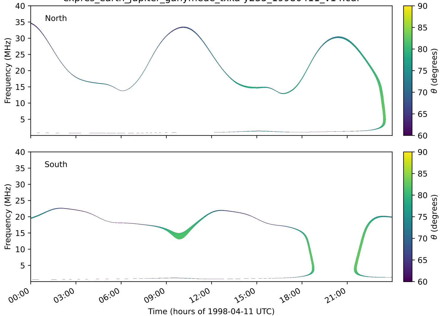
expres_earth_jupiter_ganymede_txka-y235_19980411_v14.cdf
