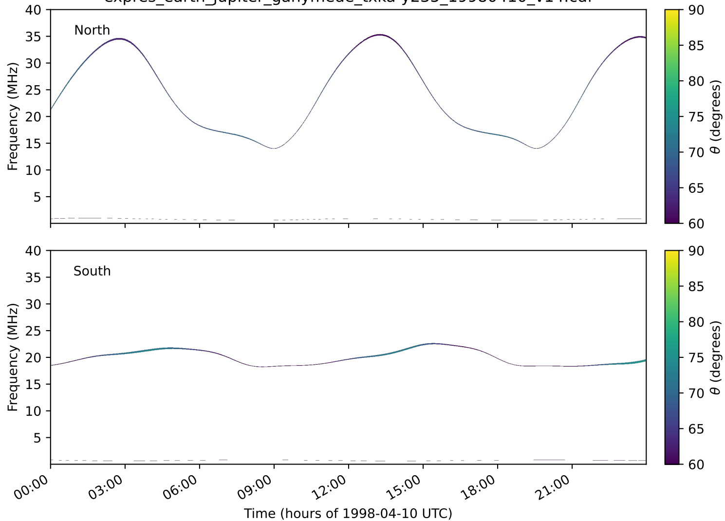
expres_earth_jupiter_ganymede_txka-y235_19980410_v14.cdf
