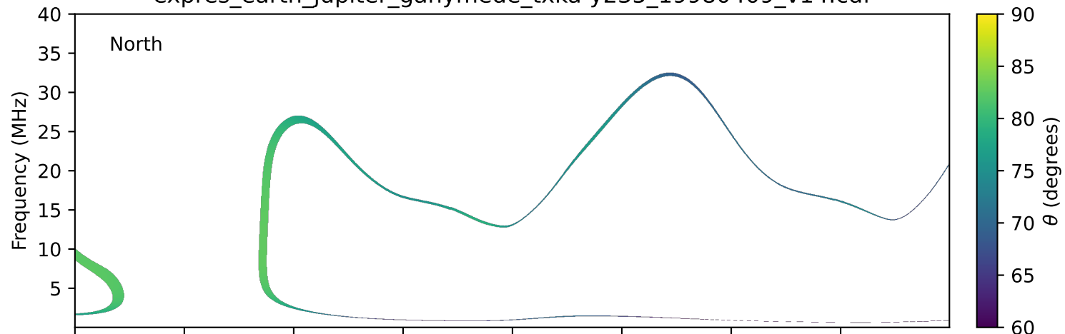
expres_earth_jupiter_ganymede_txka-y235_19980409_v14.cdf
