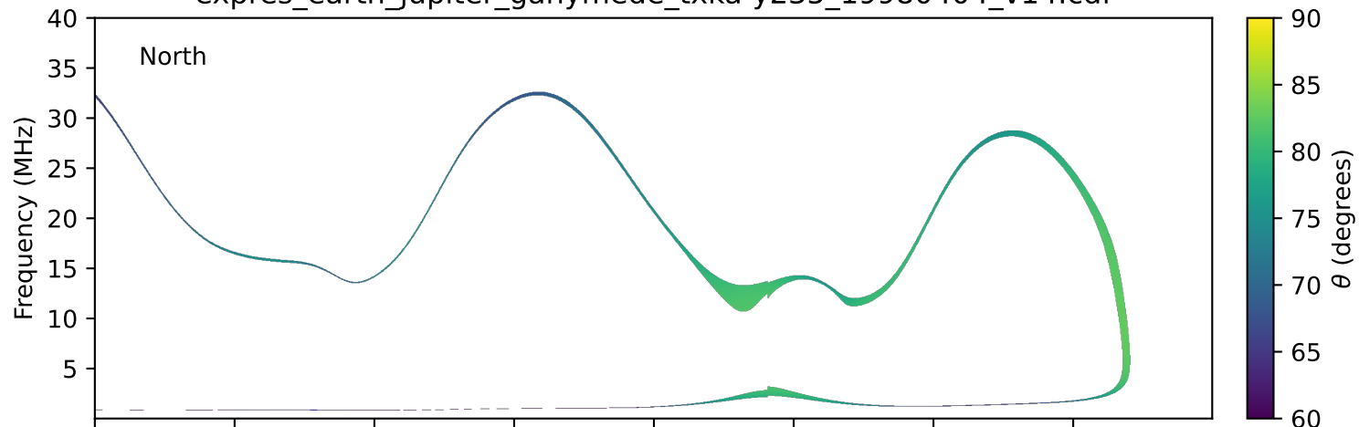
expres_earth_jupiter_ganymede_txka-y235_19980404_v14.cdf
