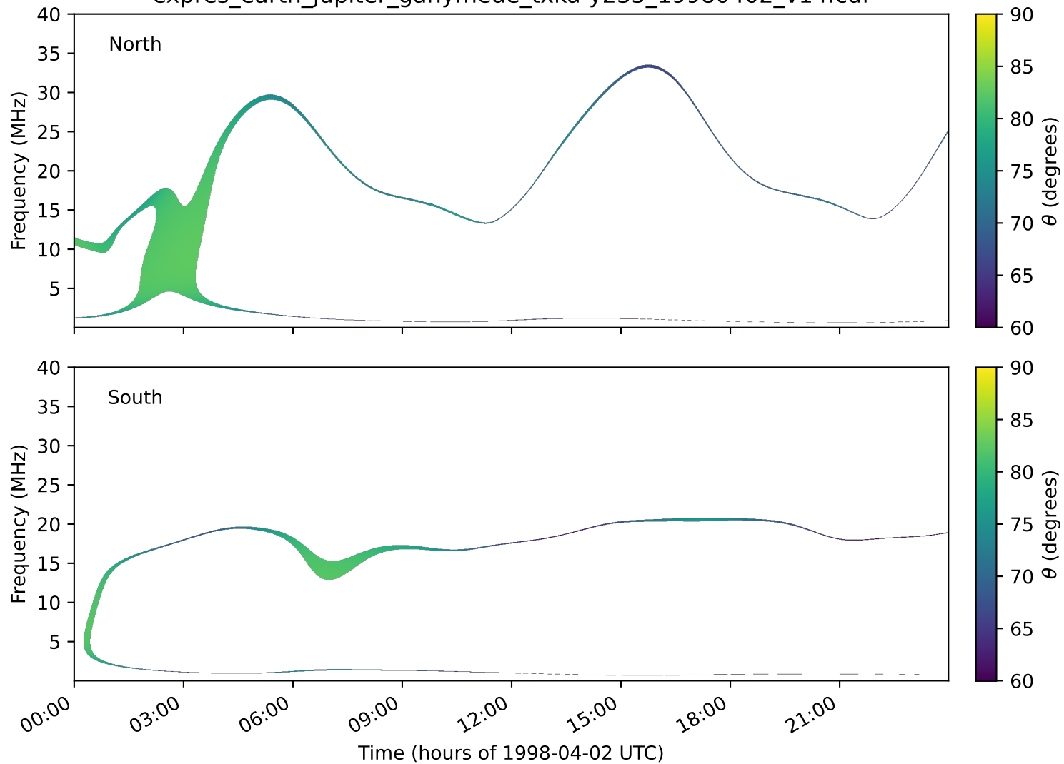
expres_earth_jupiter_ganymede_txka-y235_19980402_v14.cdf
