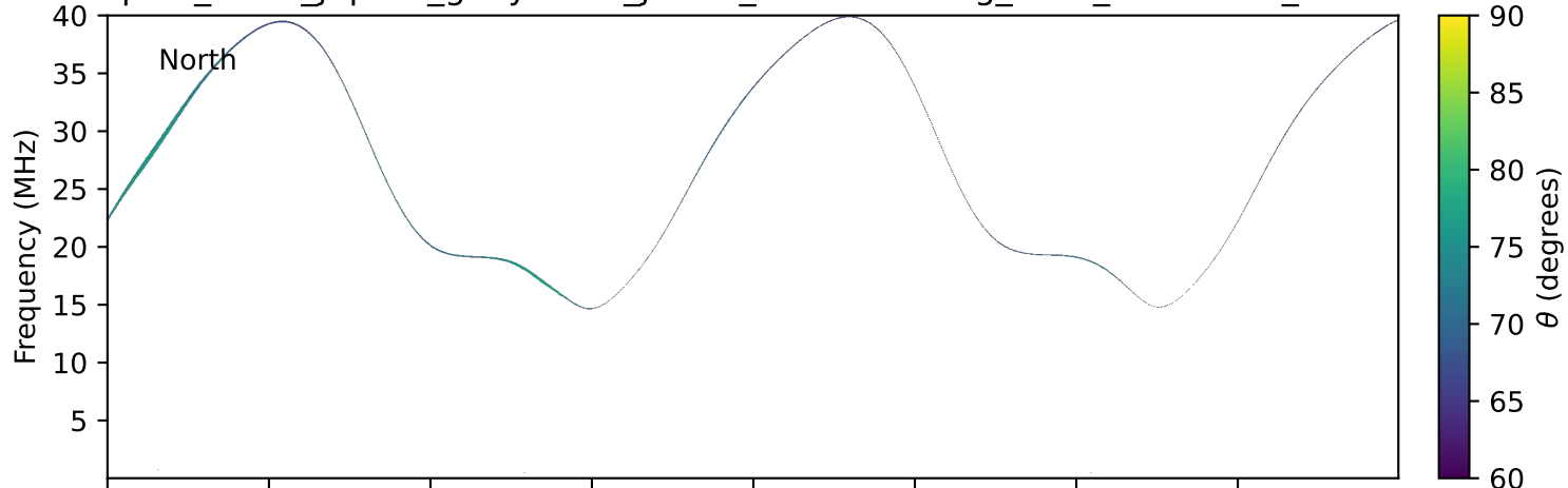
expres_earth_jupiter_ganymede_jrm33_lossc-wid1deg_3kev_19980417_v11.cdf
