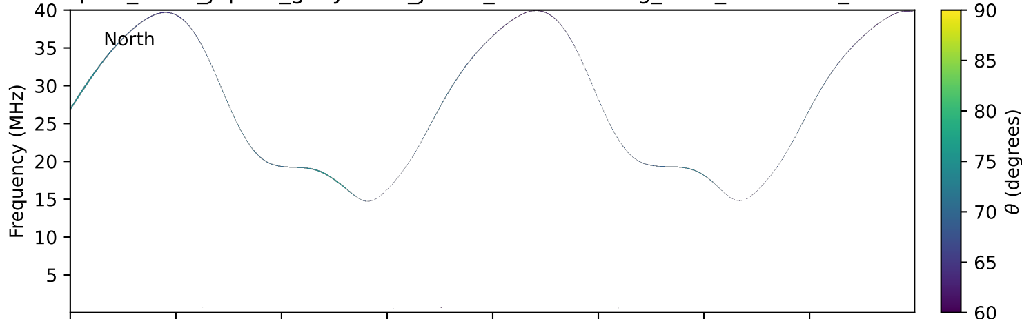
expres_earth_jupiter_ganymede_jrm33_lossc-wid1deg_3kev_19980410_v11.cdf
