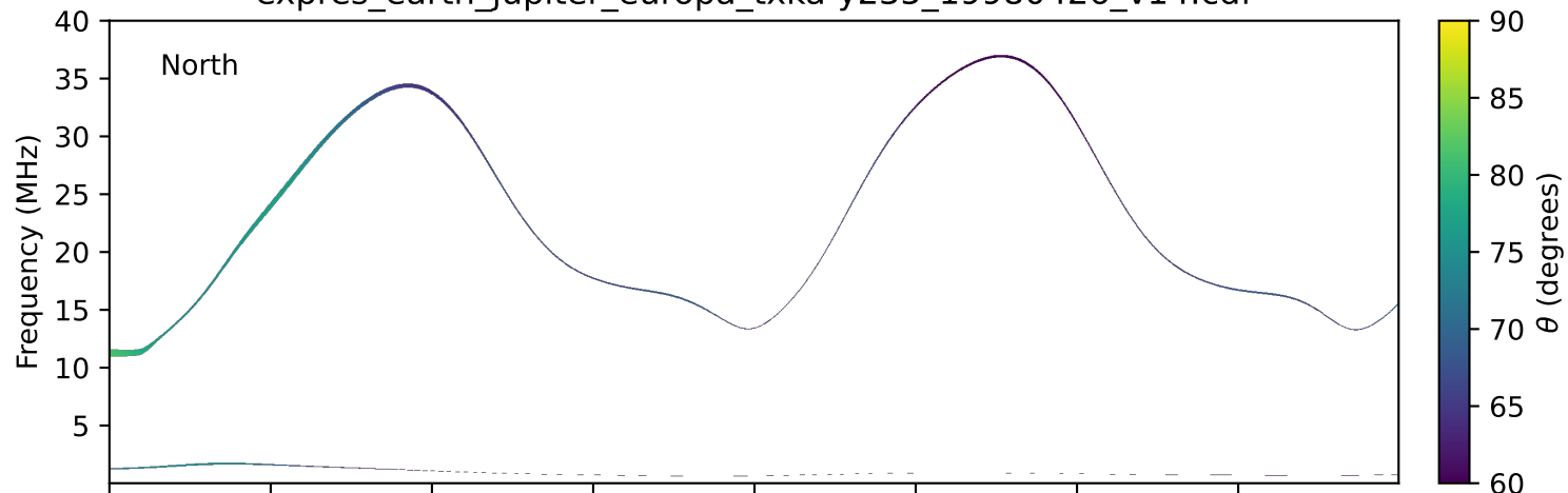
expres_earth_jupiter_europa_txka-y235_19980426_v14.cdf
