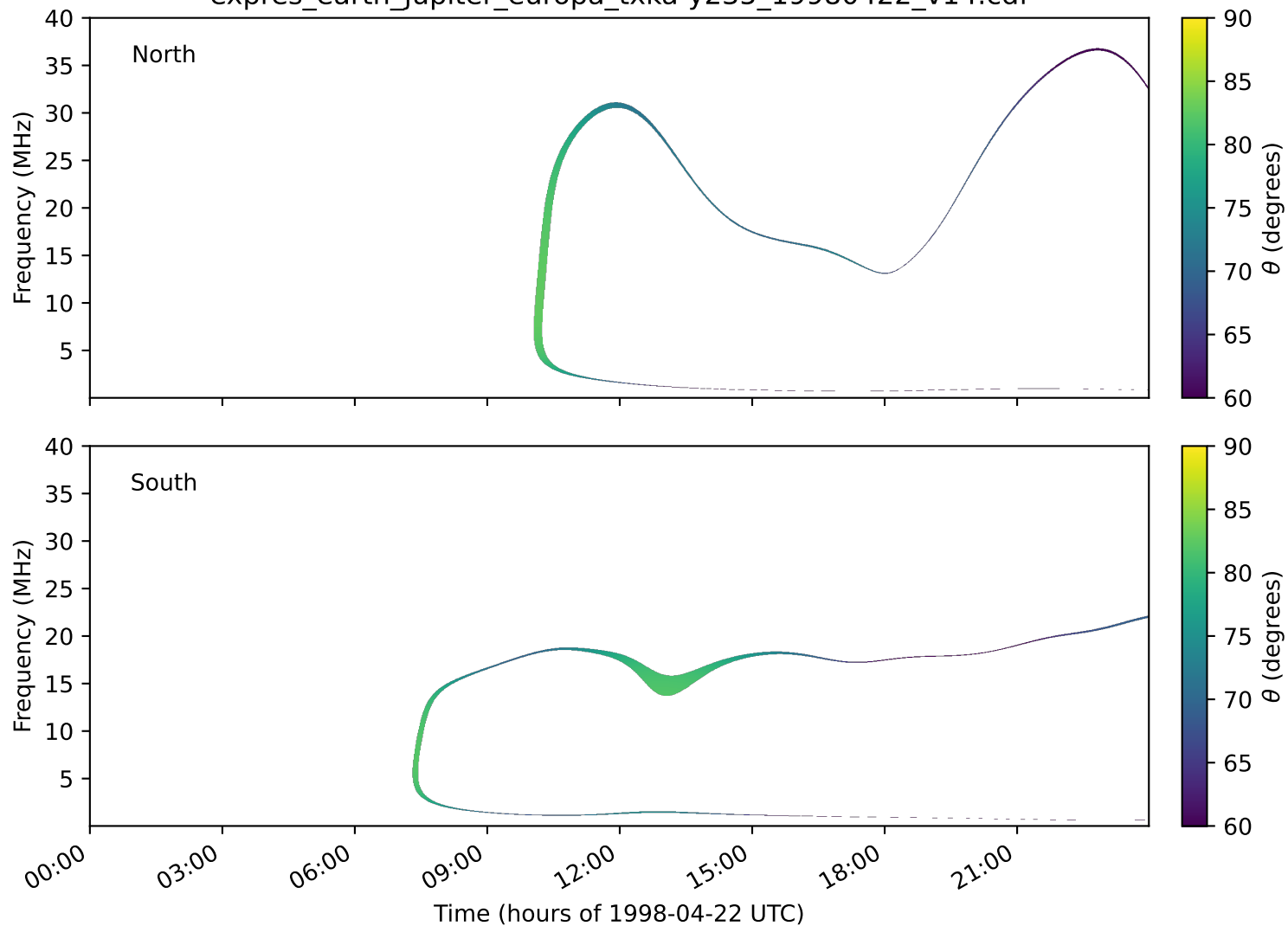
expres_earth_jupiter_europa_txka-y235_19980422_v14.cdf
