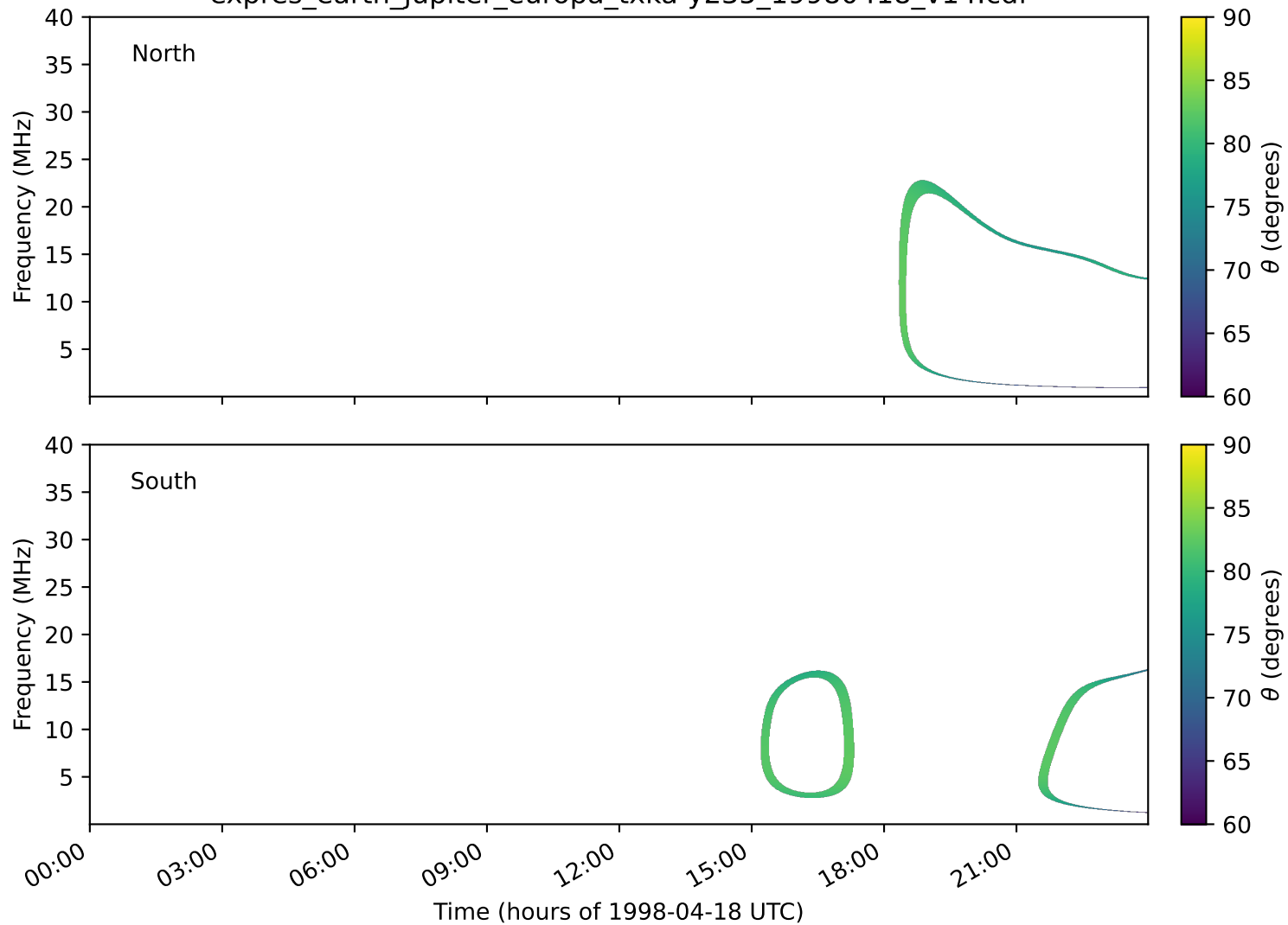
expres_earth_jupiter_europa_txka-y235_19980418_v14.cdf
